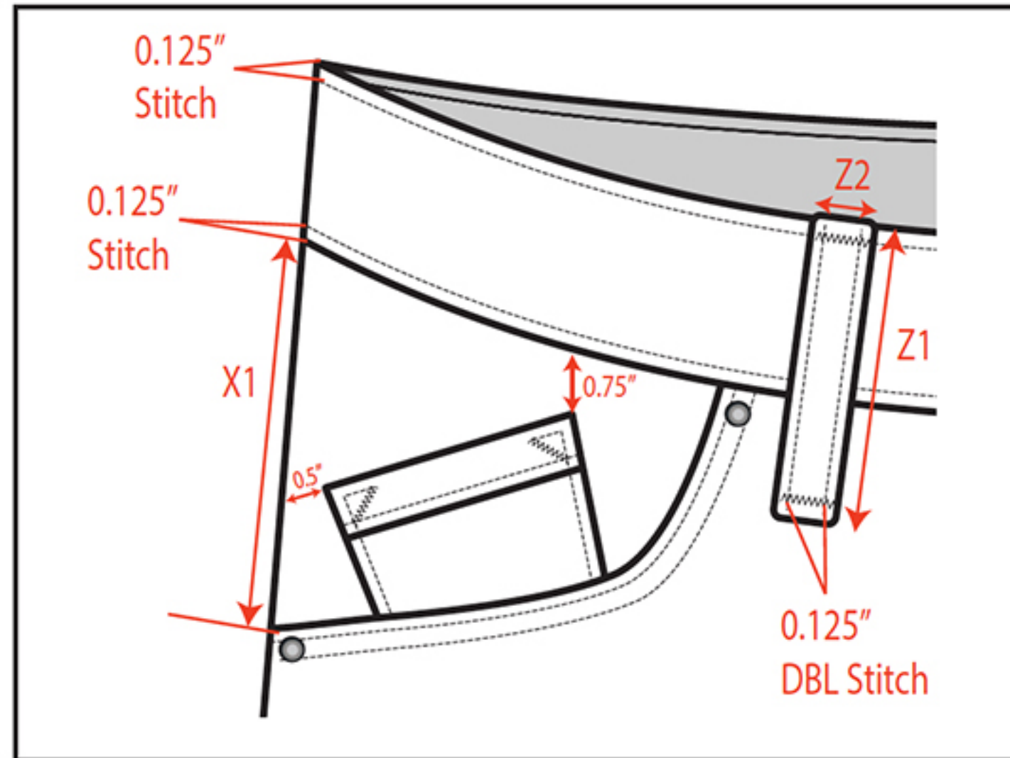
Front Side Pocket Detail
