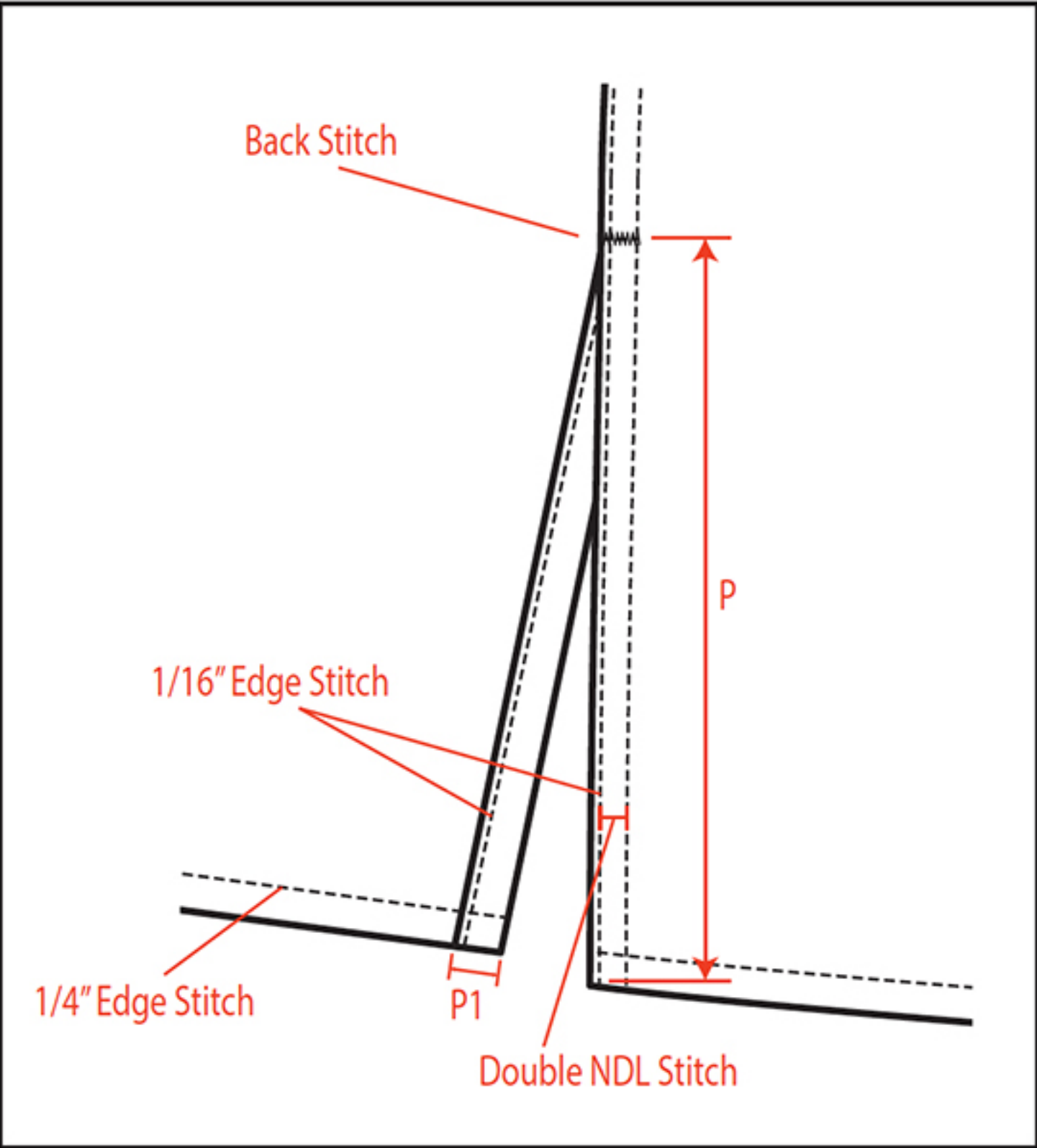
Side Slit Detail
