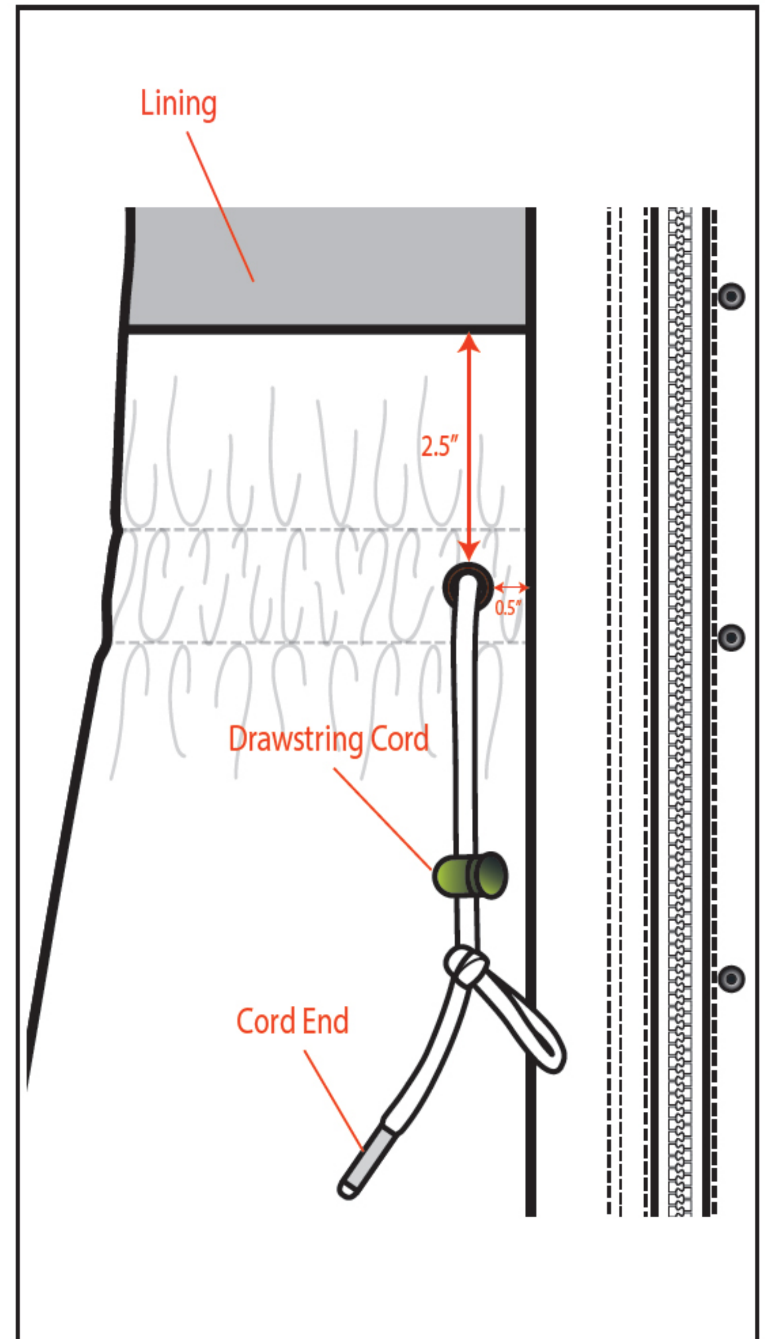
Front Zipper Detail (Inside View)
