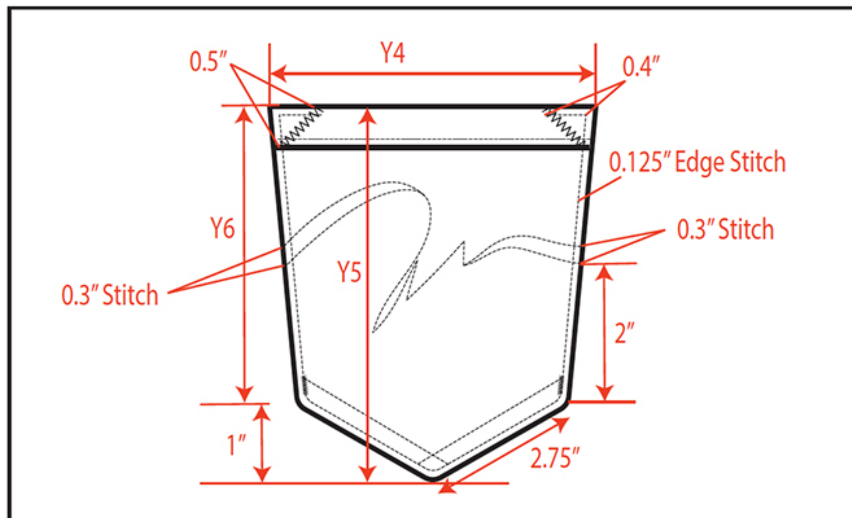
Back Pocket Detail (right side / mirror placement see previous page)
