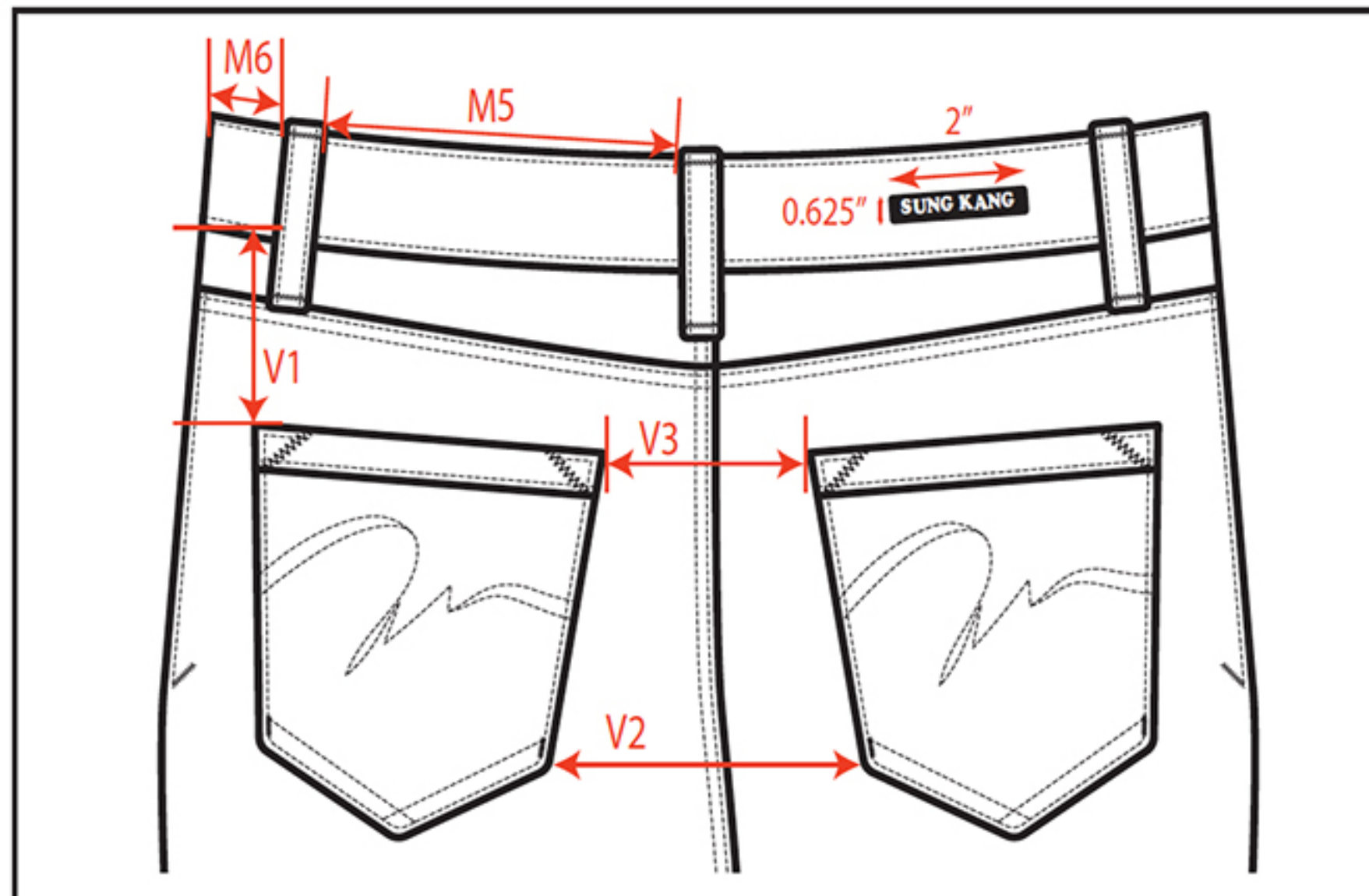
Back Waist Detail
