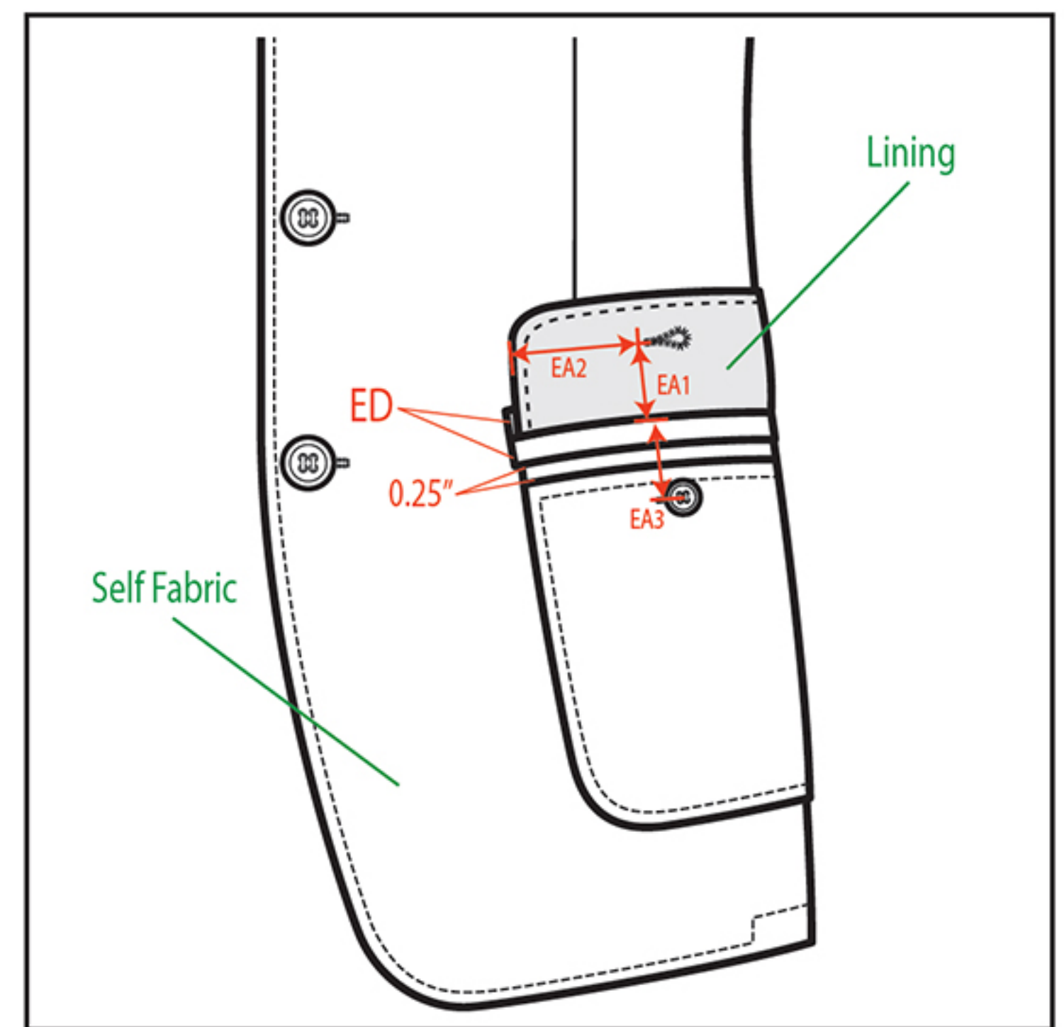
Button / Pocket Detail
