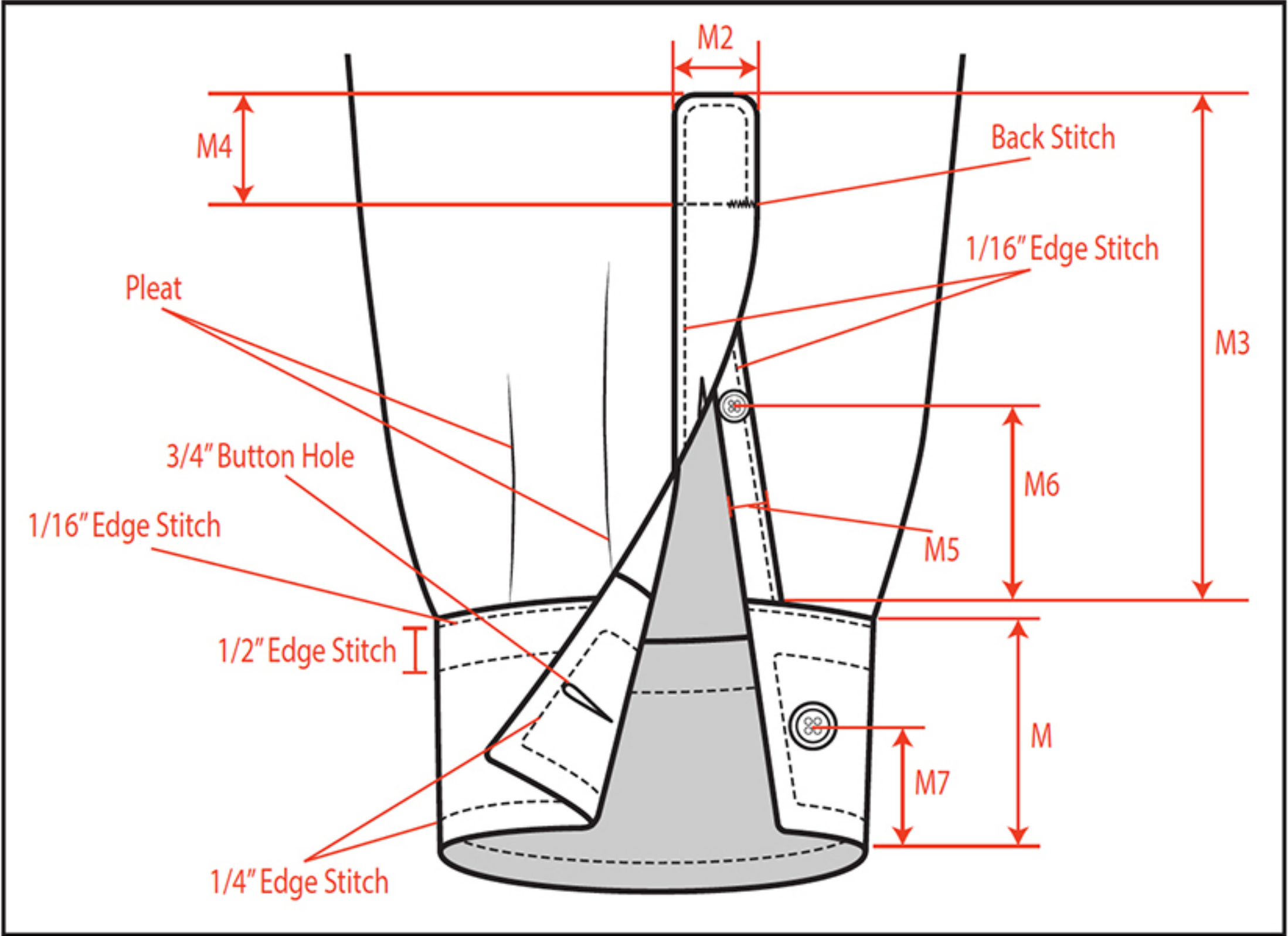
Sleeve Cuff Detail
