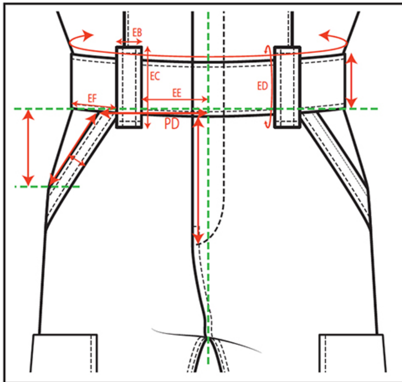
Side Pocket Detail
