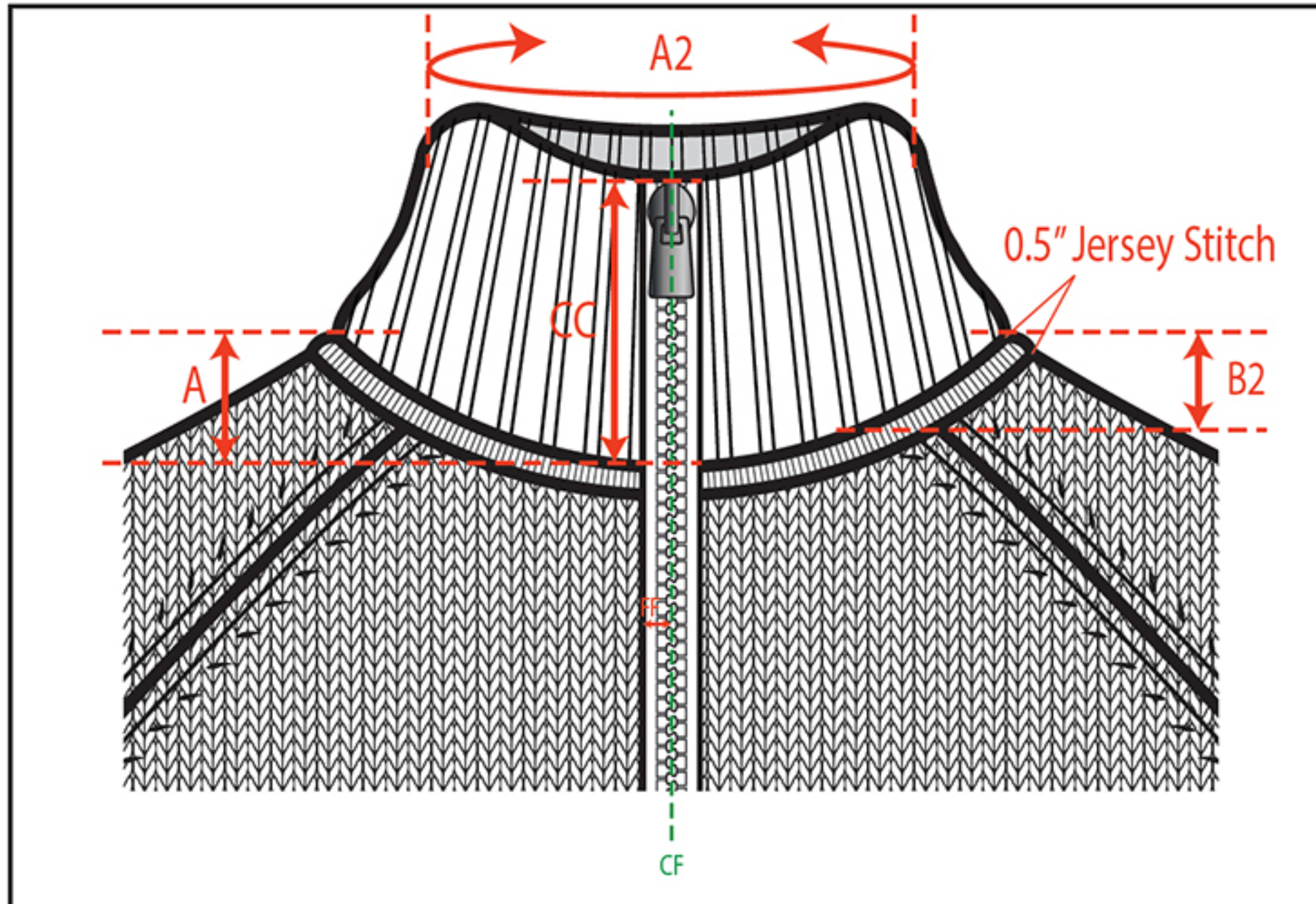
Collar Detail (zipper pull up)
