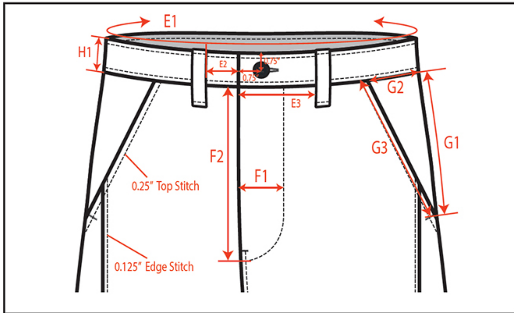
Front Waist Detail
