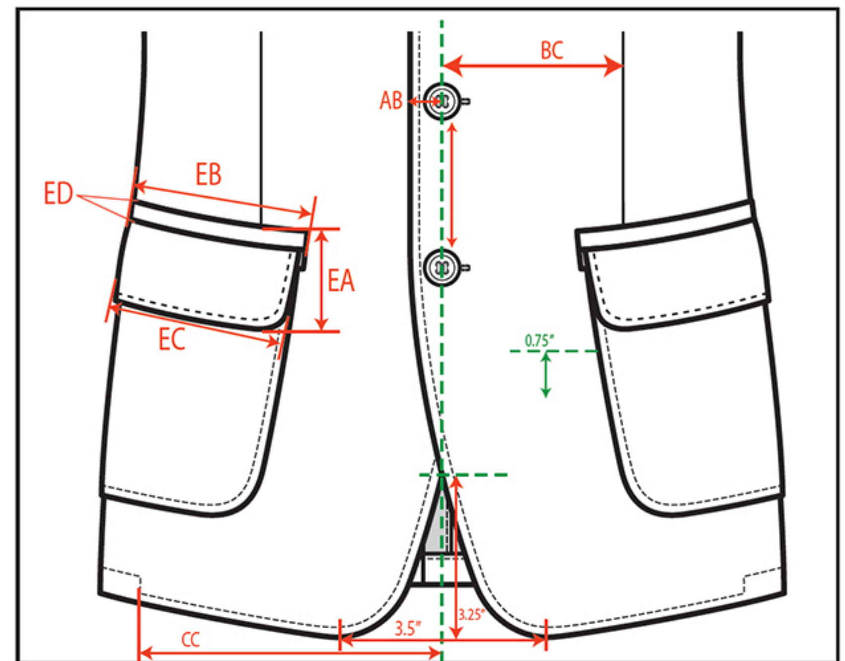
Button / Pocket Detail
