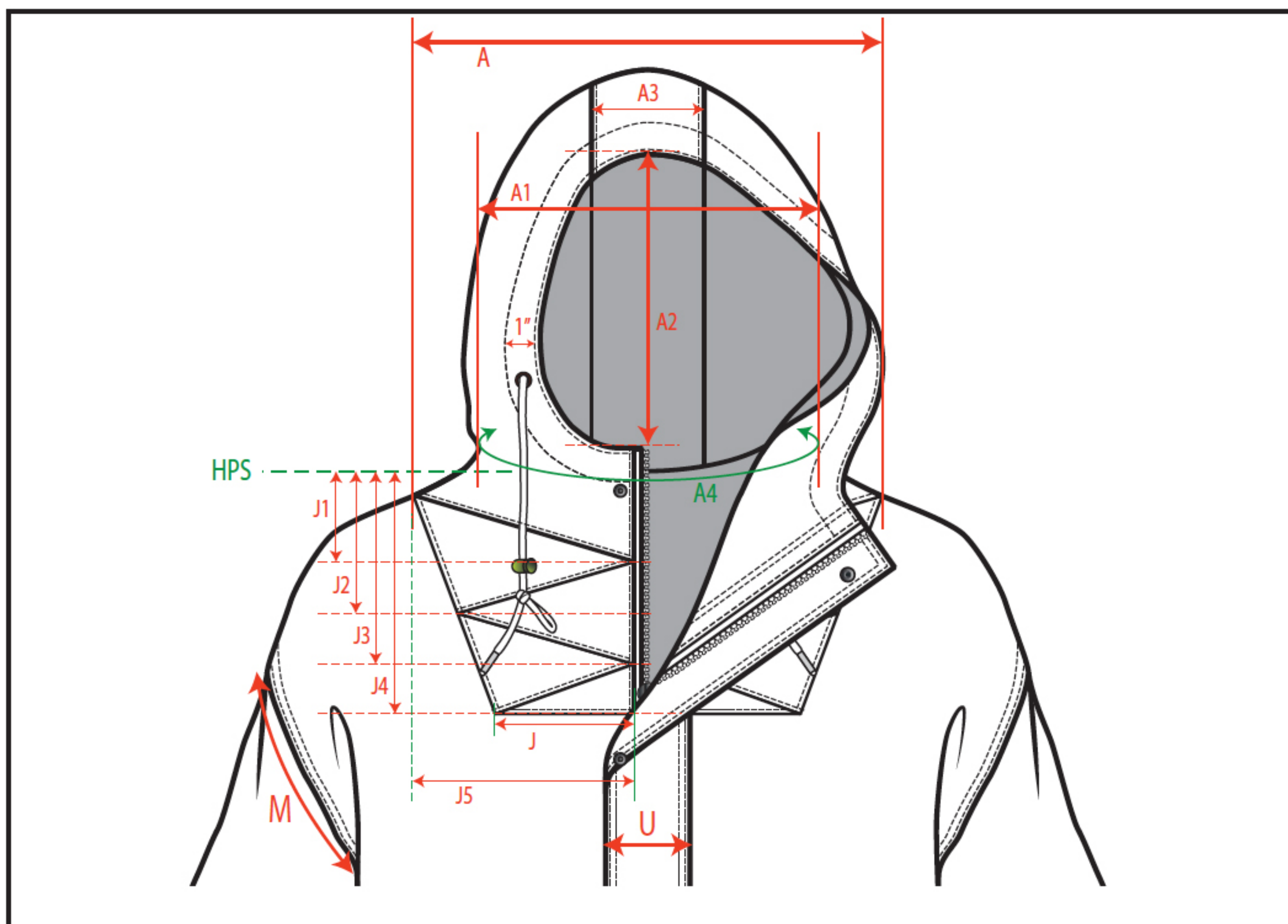
Front & Hood Detail
