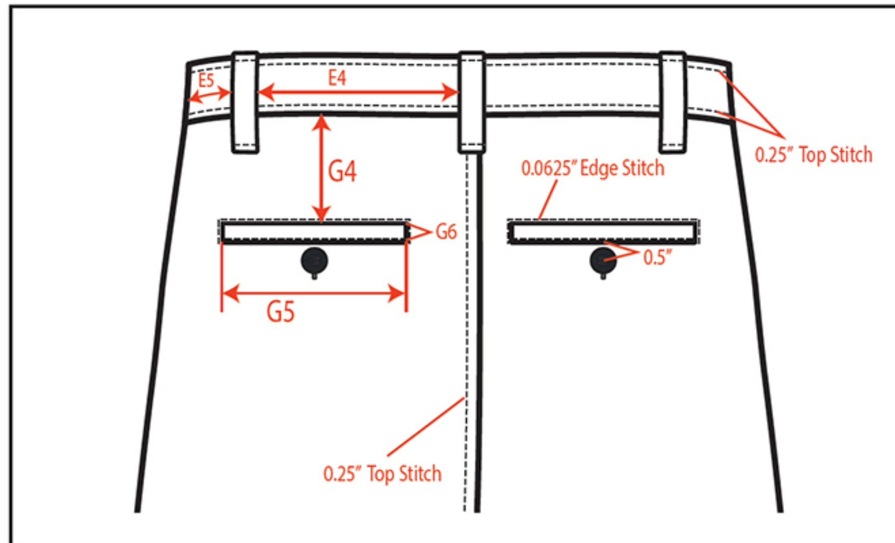
Back Waist Detail
